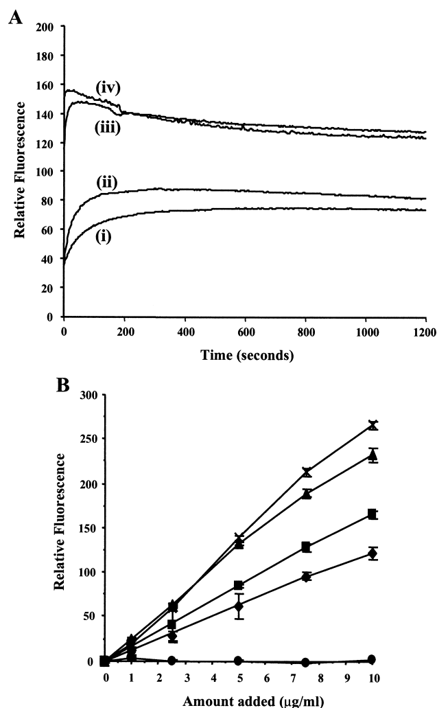
Fig. 1. (A) Rate of reaction between fluorescamine and pLL under different pH conditions. Fluorescamine was added to pLL (5 \mu\text{g/ml} ) in 100 mM boric acid-NaOH at pH 7.0 (i), pH 8.0 (ii), pH 9.0 (iii) and pH 9.5 (iv) and the fluorescence signal ( \lambda_{\text{ex}} 392 nm, \lambda_{\text{em}} 480 nm) was recorded over 1200 s. (B) Linearity of the fluorescamine reaction with pLL. Fluorescamine was added to pLL in 100 mM boric acid-NaOH at pH 7.0 (diamonds), pH 8.0 (squares), pH 9.0 (triangles) and pH 9.5 (crosses) and to CT DNA in 100 mM boric acid-NaOH at pH 9.5 (circles) at the indicated concentrations. Data represent the means of triplicate samples \pm S.D.
